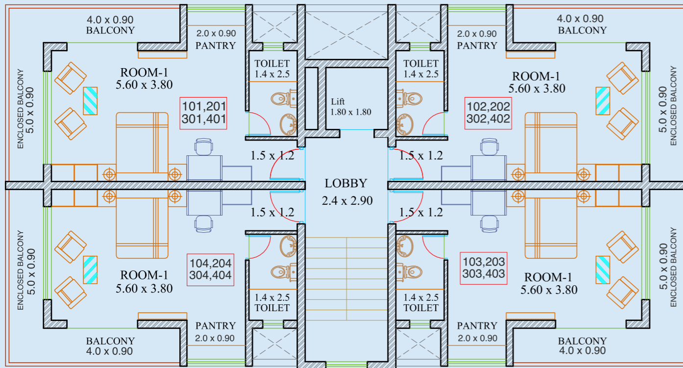
Area - 48.0 Sq.Mtrs / 516.67 Sq.FT. TYPICAL FIRST, SECOND, THIRD, FORTH FLOOR PLAN
