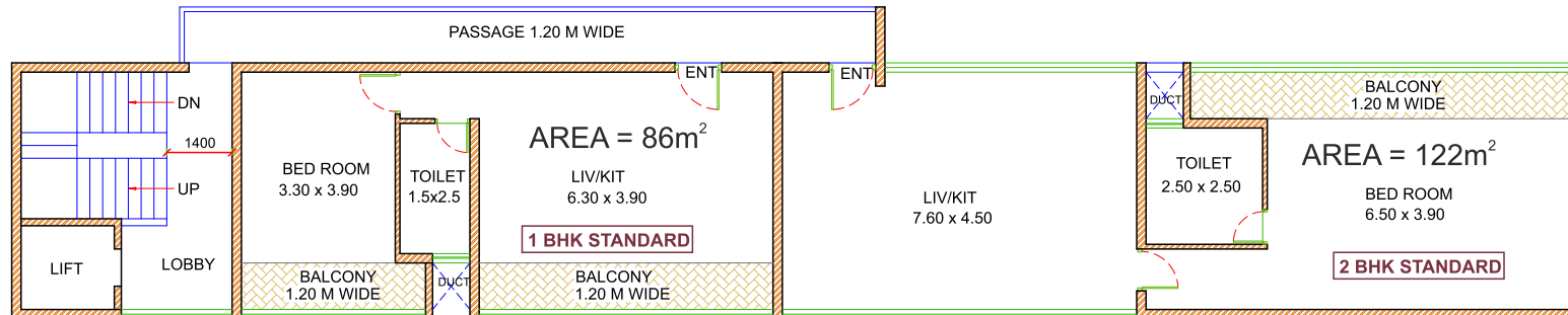
2ND FLOOR & 4TH FLOOR PLAN
