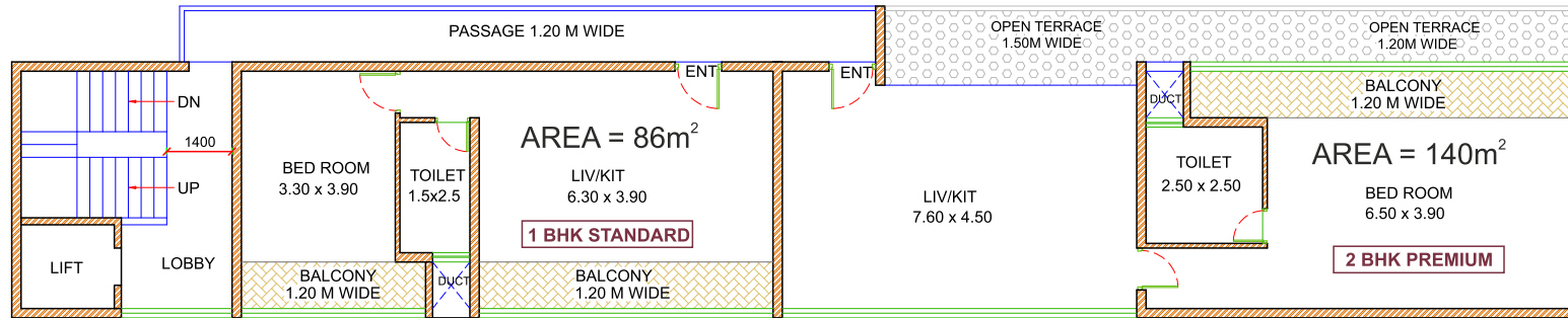
1ST FLOOR & 3RD FLOOR PLAN
